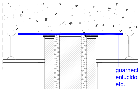
Detalle ESV-02.c-R5
